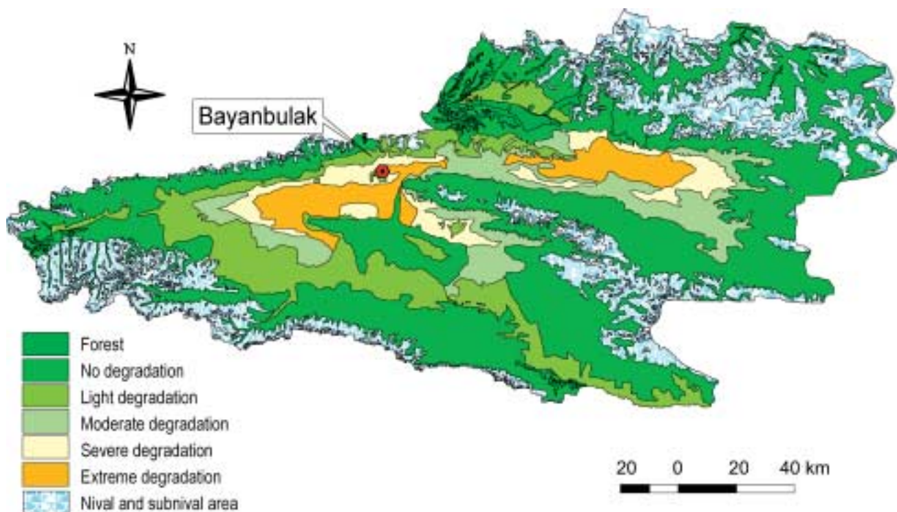
FIGURE 4 Distribution of degraded pastureland in the Bayanbulak region
