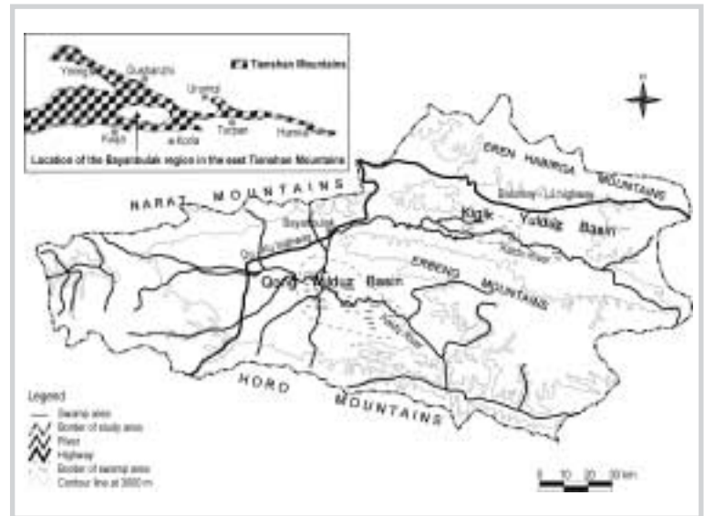
FIGURE 1 Sketch map of the Bayanbulak region in the eastern Tianshan Mountains.
