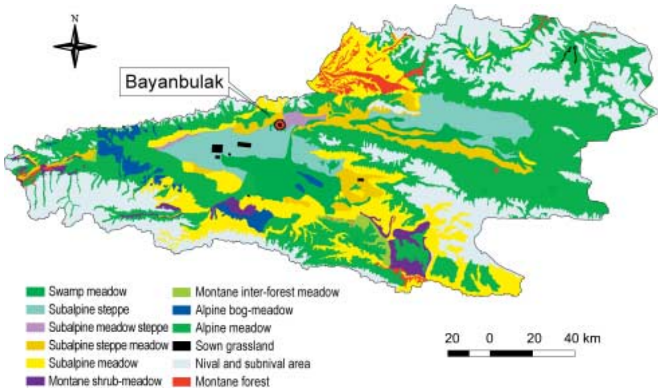
FIGURE 2 Grassland types and their distribution in the Bayanbulak region.
